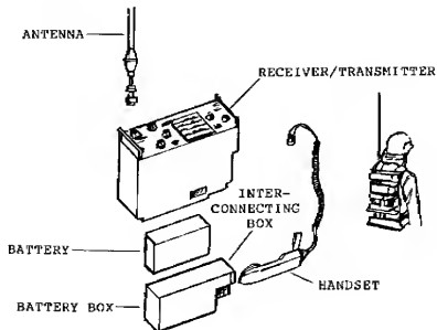
Figure 2-31. AN/PRC-119 radio.
